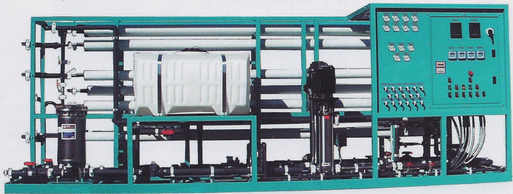
MODEL DELTA-20 28,800 GPD of High Purity Water
